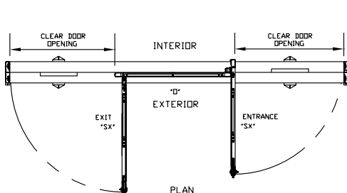
BYPASS DOOR SYSTEM RIGHT HAND ENTRY
