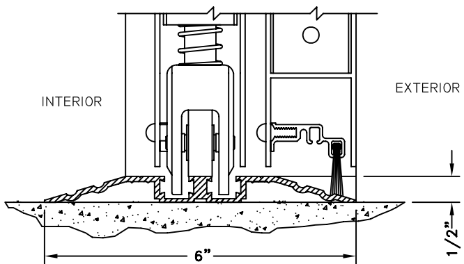
THRESHOLD-TAPERED EXTRUSION 4 1/2" FRAME (DOUBLE BEVEL THROUGHOUT DOOR OPENING)
