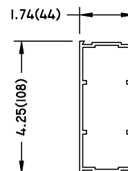
4 1/4" EXTRUSION MUNTIN BAR
