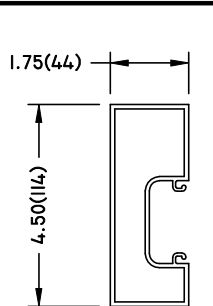
STANDARD JAMB-4 1/2"
