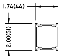
STANDARD 2" MUNTIN BAR
