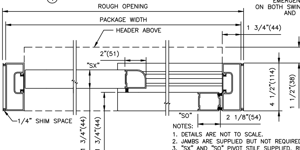
② HORIZONTAL SECTION
