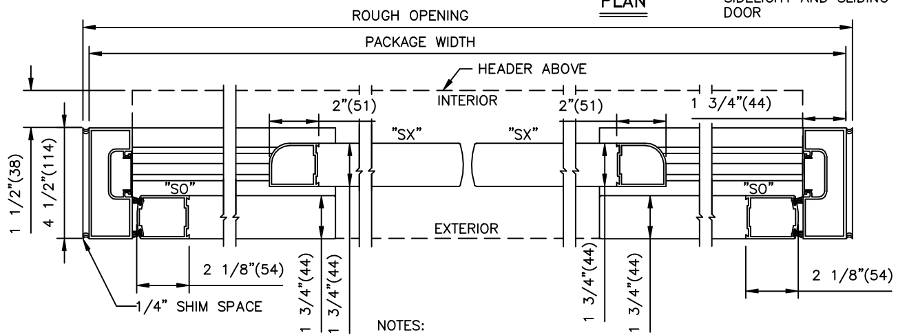
② HORIZONTAL SECTION
