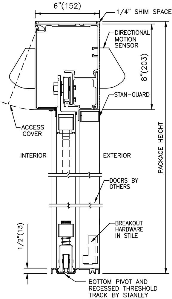
① VERTICAL SECTION
